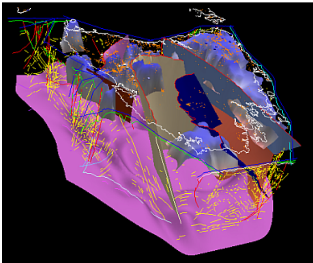
Figure 3. Indexed faceted (fault planes and geological boundaries), lines (coastline and interpreted seismic) and points (gold localities) in the Tasmanian model.
