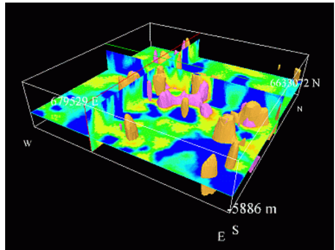
Figure 4. Slices through a 3D grid of geophysical data from the Gawler model. 3D indexed faceted volumes and reference coordinates and compass markers are also shown.
